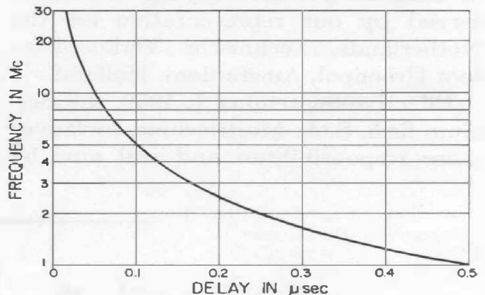
Figure 2. Plot of frequency vs. delay setting.
