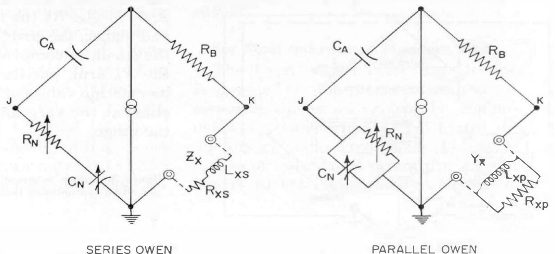
Figure 2. Elementary schematic of the Owen bridge circuits used in the Type 1632-A Inductance Bridge.
