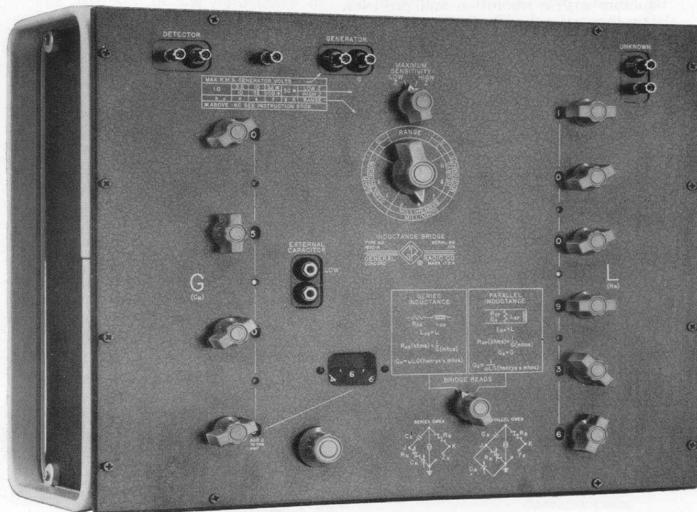
Figure 1. Panel view of the Type 1632-A Inductance Bridge.
