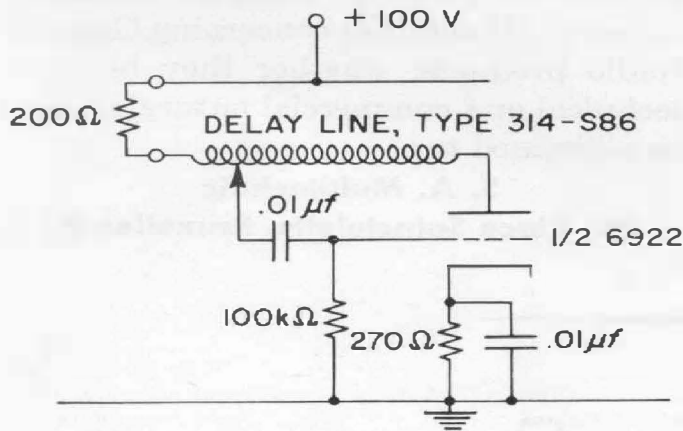
Figure 1. Schematic of the delay-line oscillator.
