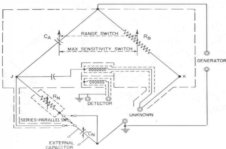
Figure 3. Bridge schematic showing the internal shielding to minimize residual-impedance errors.
